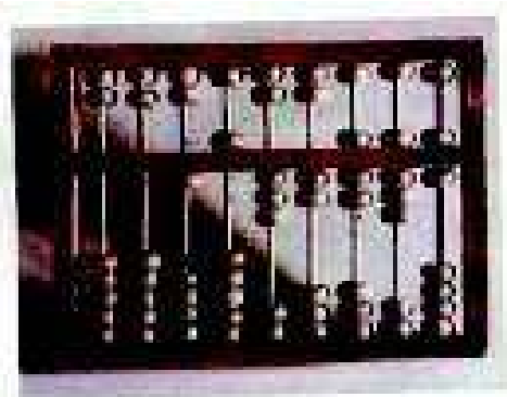
Figure 12-1 An Abacus
